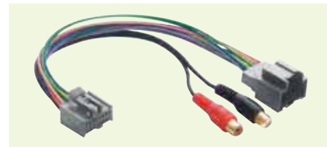
4/102 AUX-IN CONNECTION
